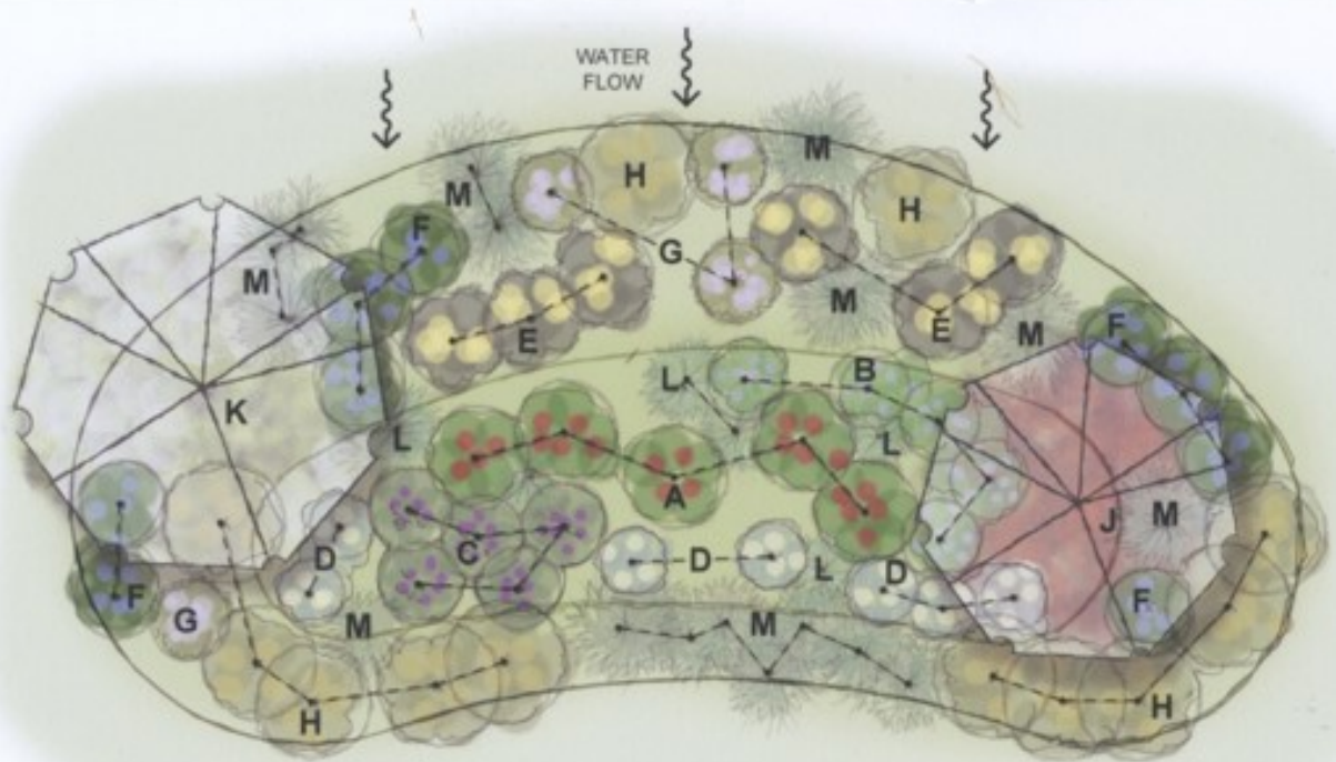
RAIN GARDEN in FULL SUN 24' x 12'
